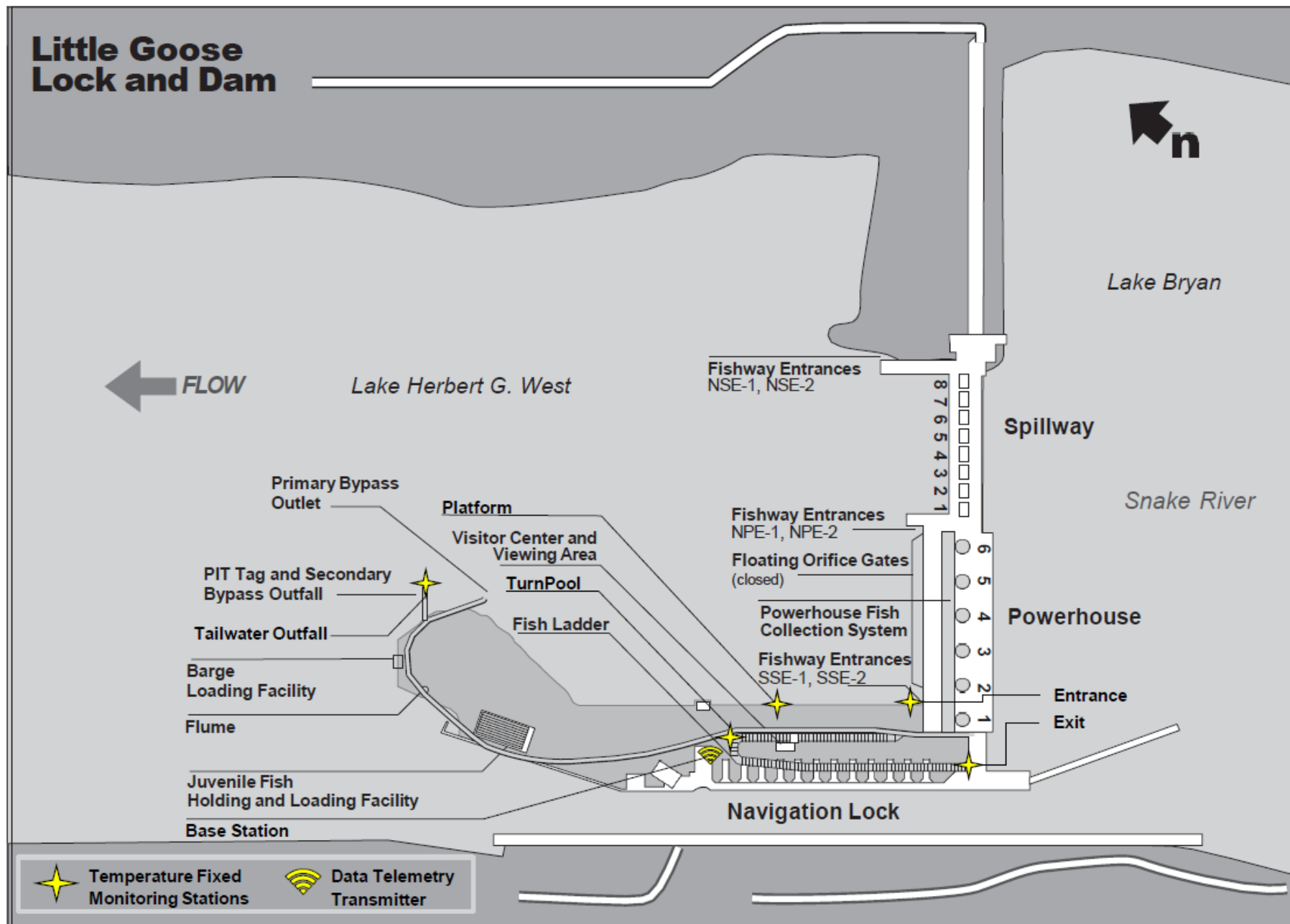
Figure LGS-1. Little Goose Lock & Dam General Site Plan. AUGUST 2024: updated ladder temperature monitoring locations.
