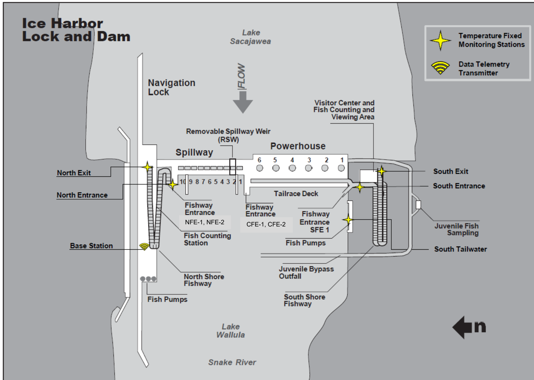
Figure IHR- 1. Ice Harbor Lock and Dam General Site Plan. AUGUST 2024: updated ladder temperature monitoring locations.
