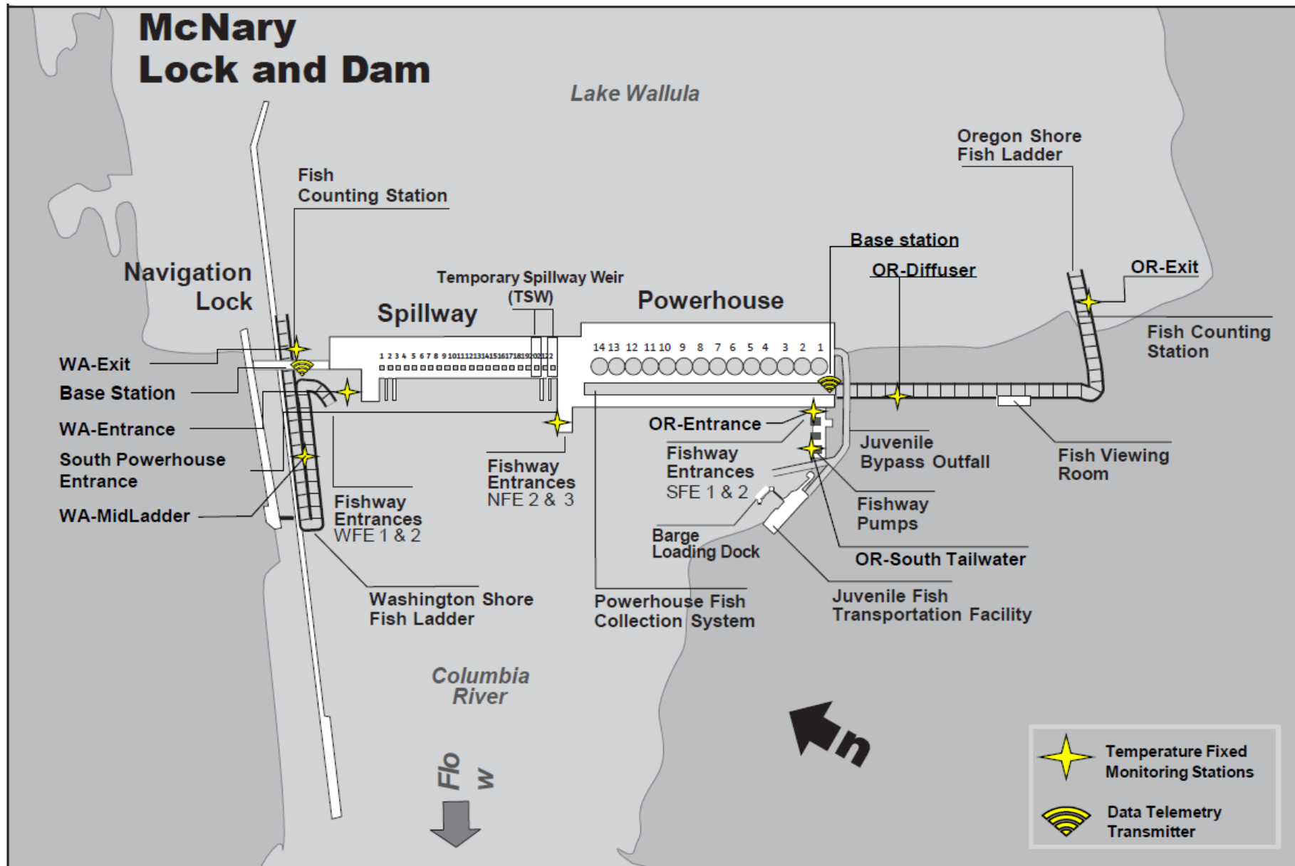
Figure MCN-1. McNary Lock & Dam General Site Plan. AUGUST 2024: updated ladder temperature monitoring locations.
