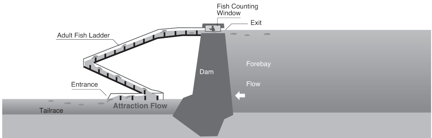
Figure OV-1 Generalized Example of Types of Fish Passage Structures at a Dam
