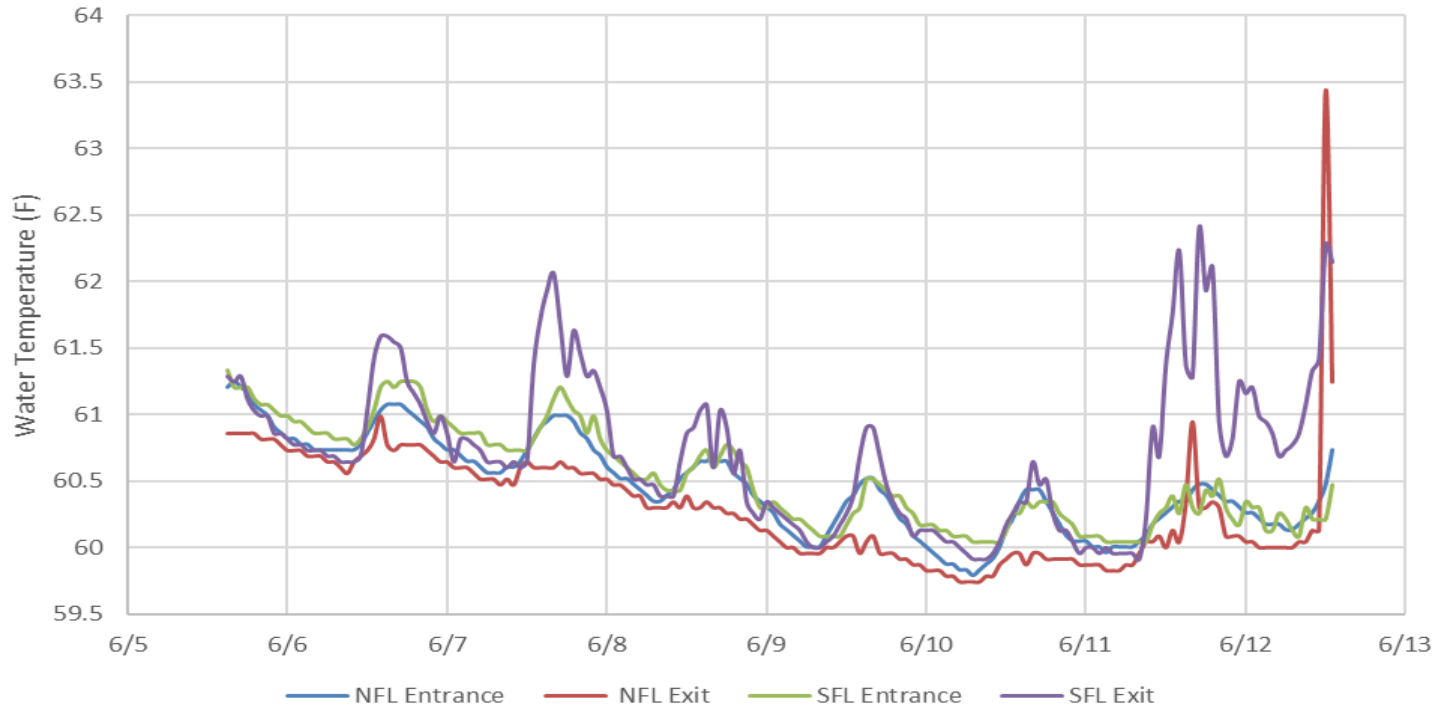
Water Temperature of JDA Fish Ladders (6/6 - 6/12)
