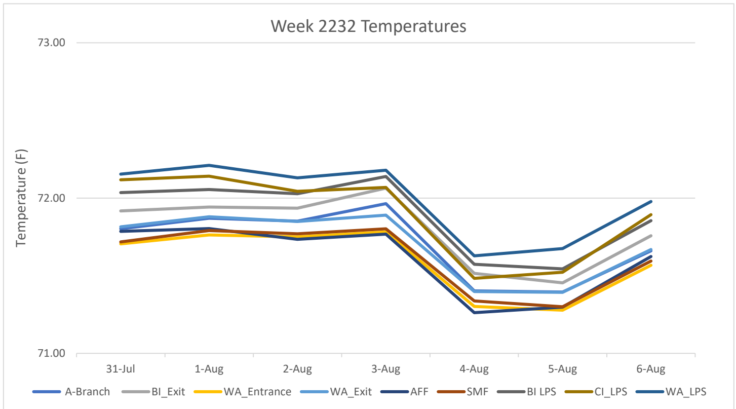
Figure 1. Average fishway temperatures for 31 July to 06 August at Bonneville Lock & Dam.
