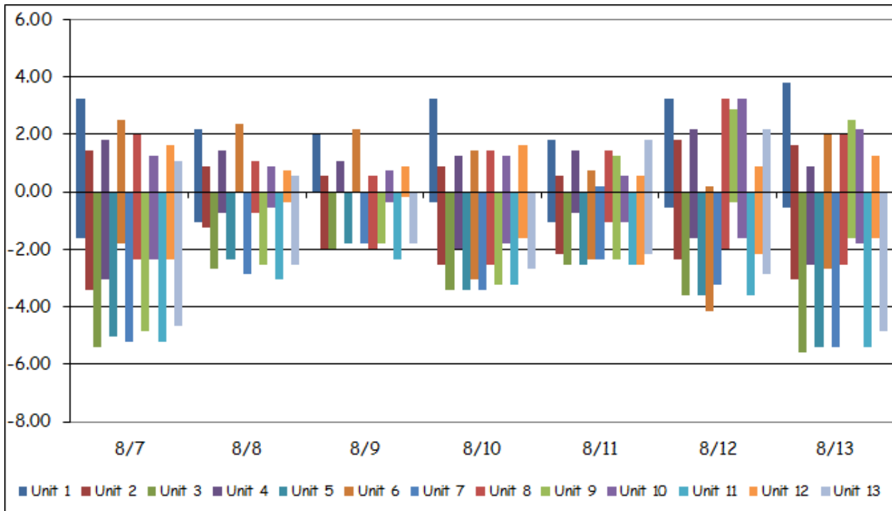
Figure 3: Average Gatewell Temperature Differentials for Units 1 - 14
