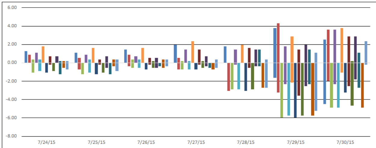
Figure 3: Average Gatewell Temperature Differentials for Units 1 - 14
