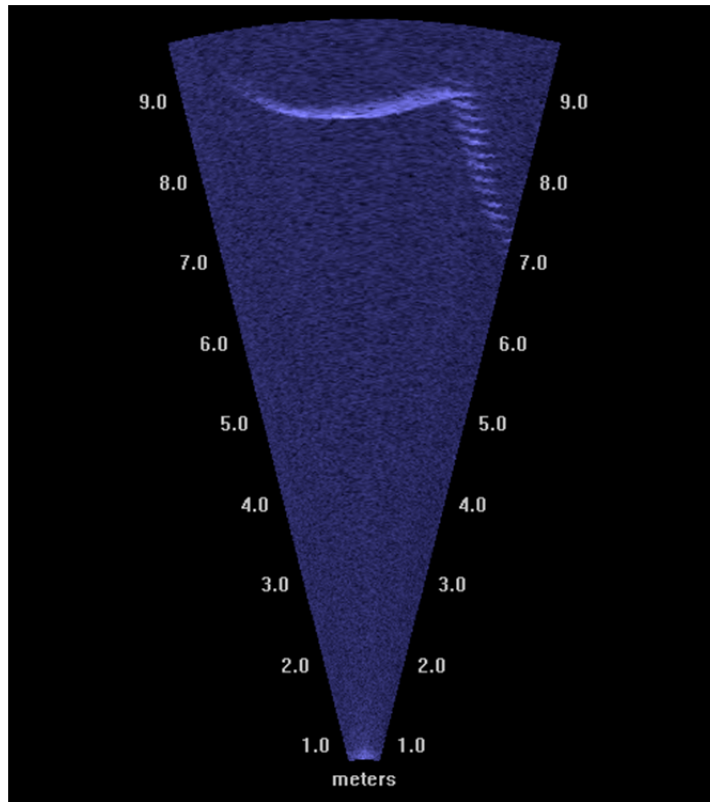
Figure 2.4. DIDSON View at Elevation 328 Showing Main Pier Nose and Trash Rack Structure
