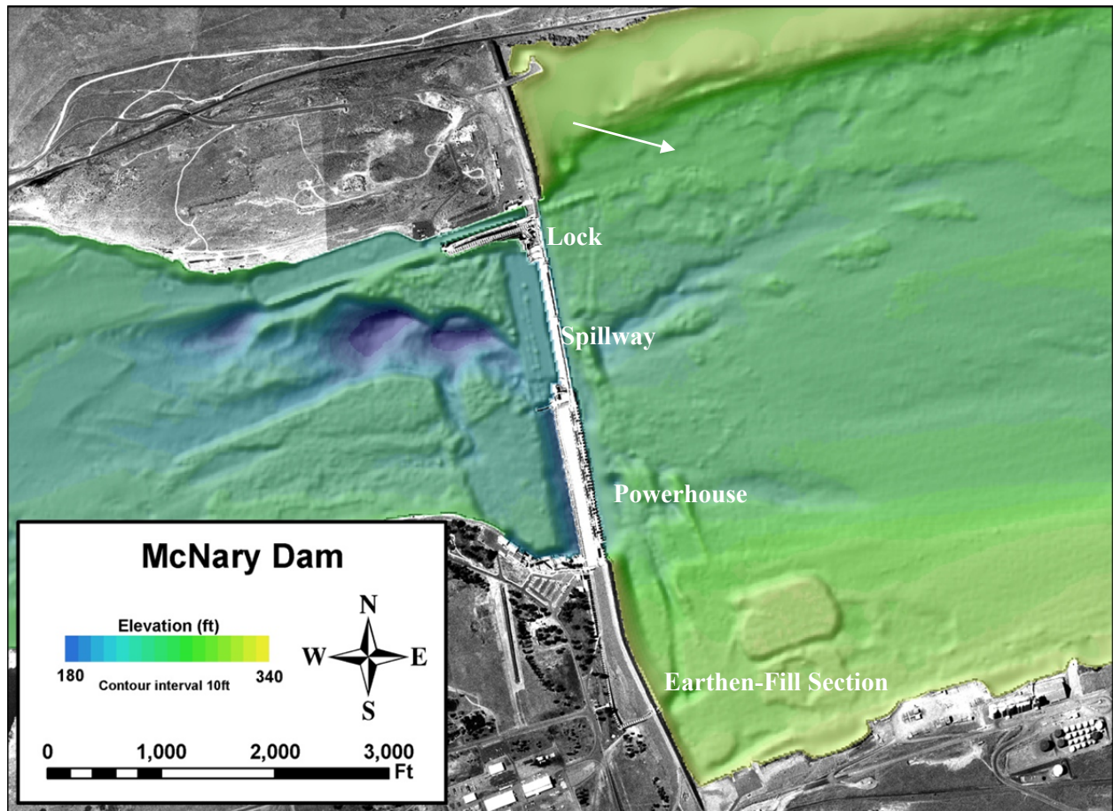
Figure 1.2. Plan View of McNary Dam Major Structural Features with River Bathymetry
