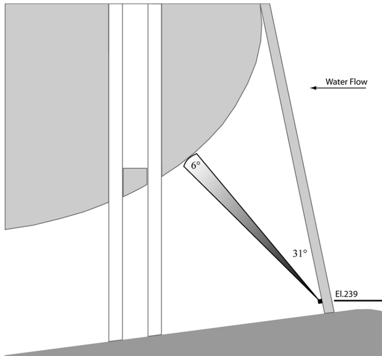
Figure 2.2. Side View of the Unit Intake Split-Beam Transducer Deployment. Each Transducer was Mounted on the Trash Rack at an Elevation of 239 ft, Aimed Downstream 31 Degrees from the Trash Rack Plane.
