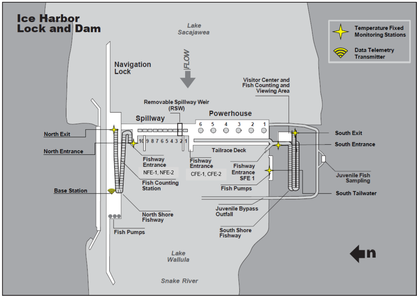
Figure IHR-1. Ice Harbor Lock & Dam General Site Plan.
