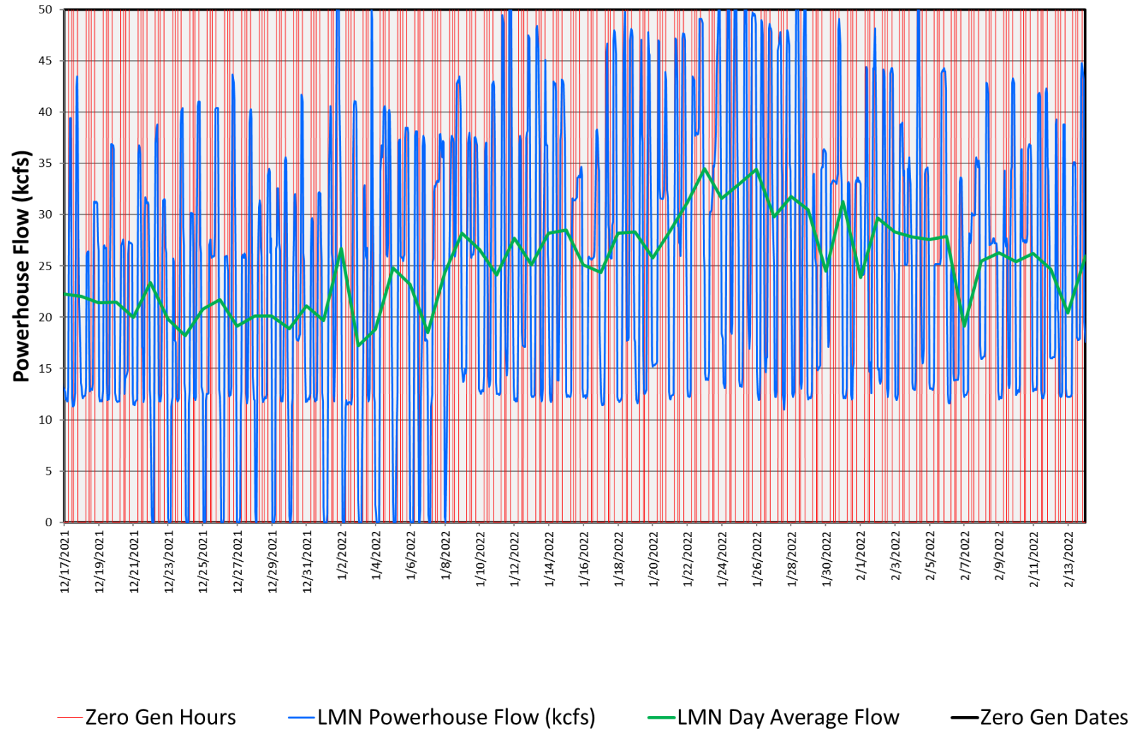
Lower Monumental Dam Zero Generation Operations
