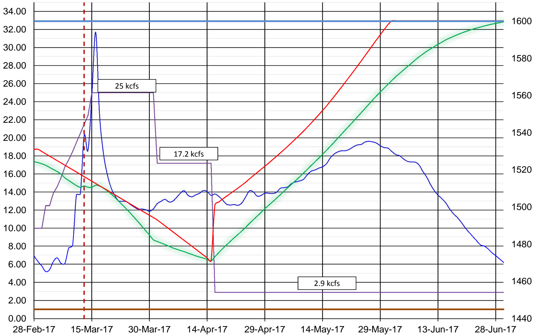
2017 2.9 MAF Dworshak April - June Operations STP
