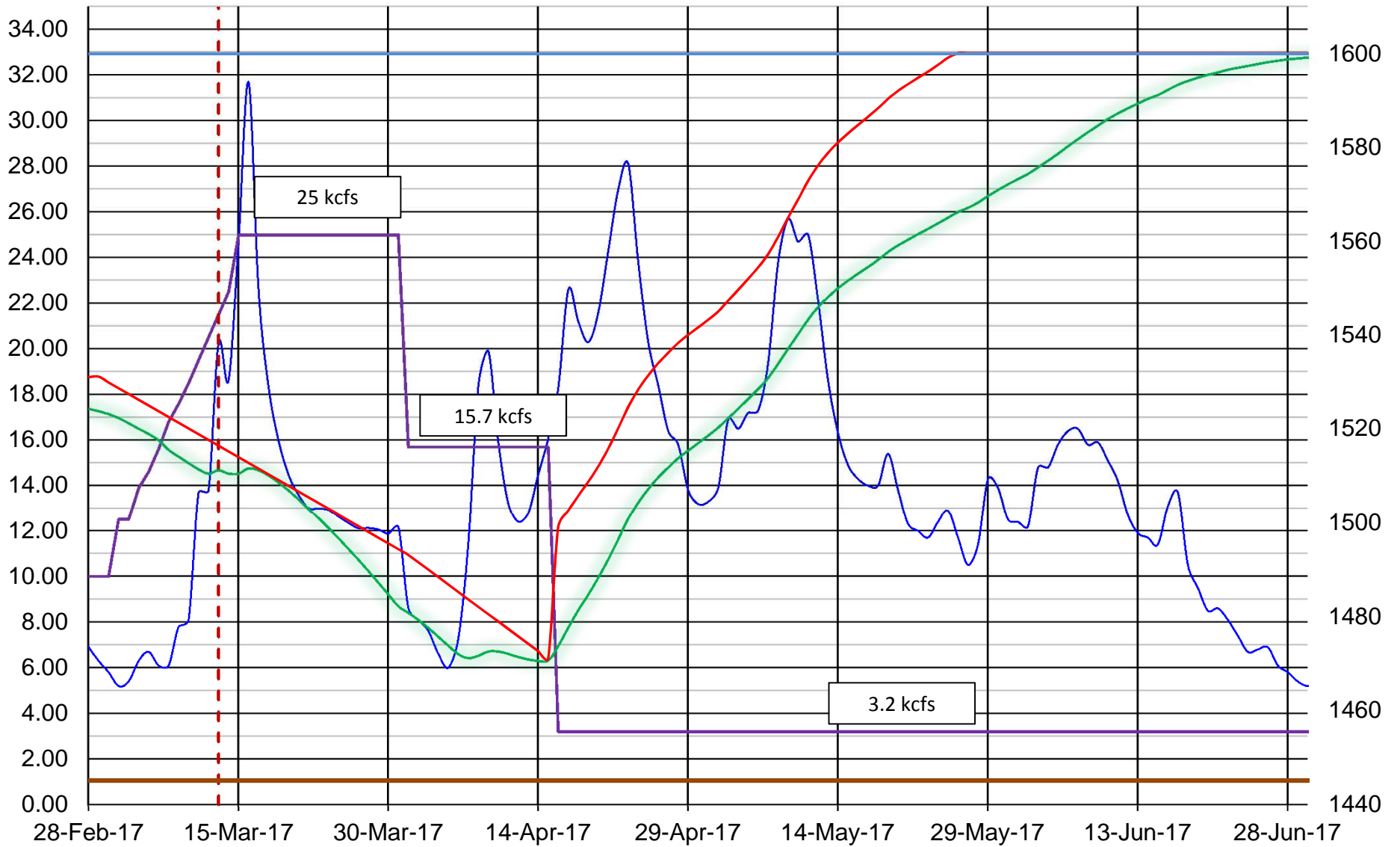
2017 2.9 MAF Dworshak April - June Operations 1989 AY (Early Runoff)
