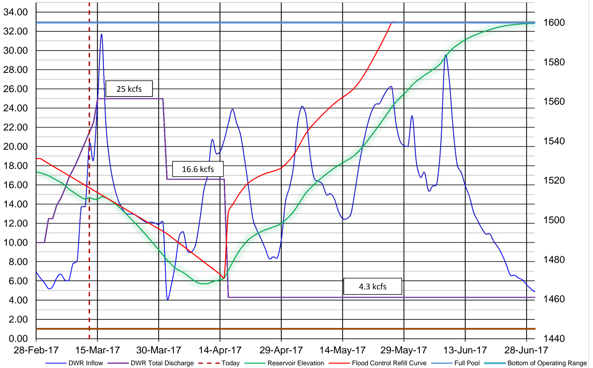
2017 2.9 MAF Dworshak April - June Operations 1985 (Late Runoff)
