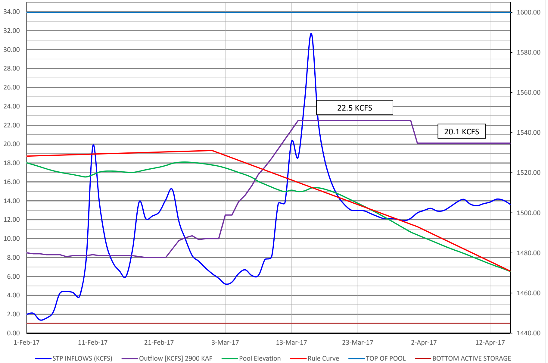
STP 22.5kcfs Dworshak 2.9 MAF 15 Apr Operation
