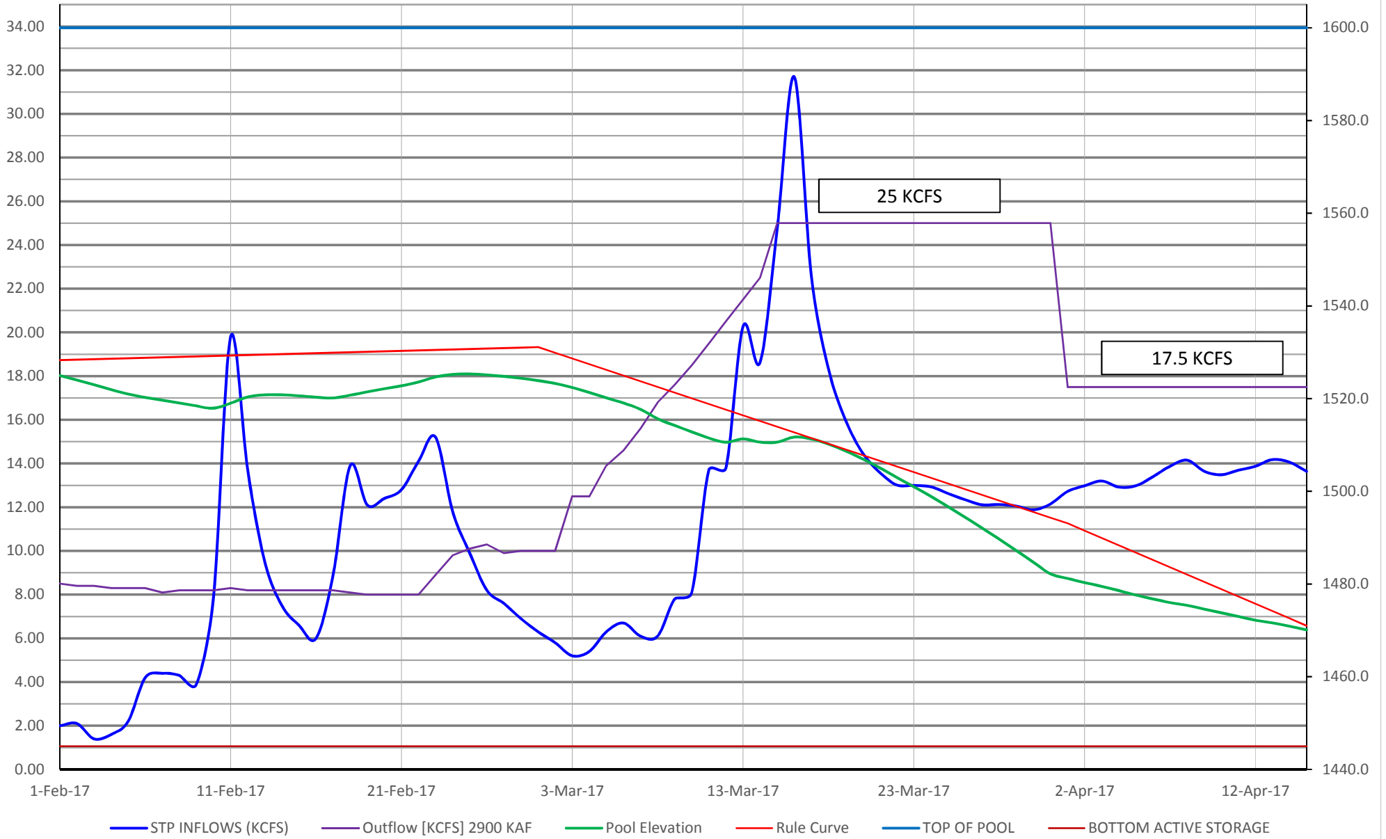
STP 25kcf through March Dworshak 2.9 MAF 15 Apr Operation
